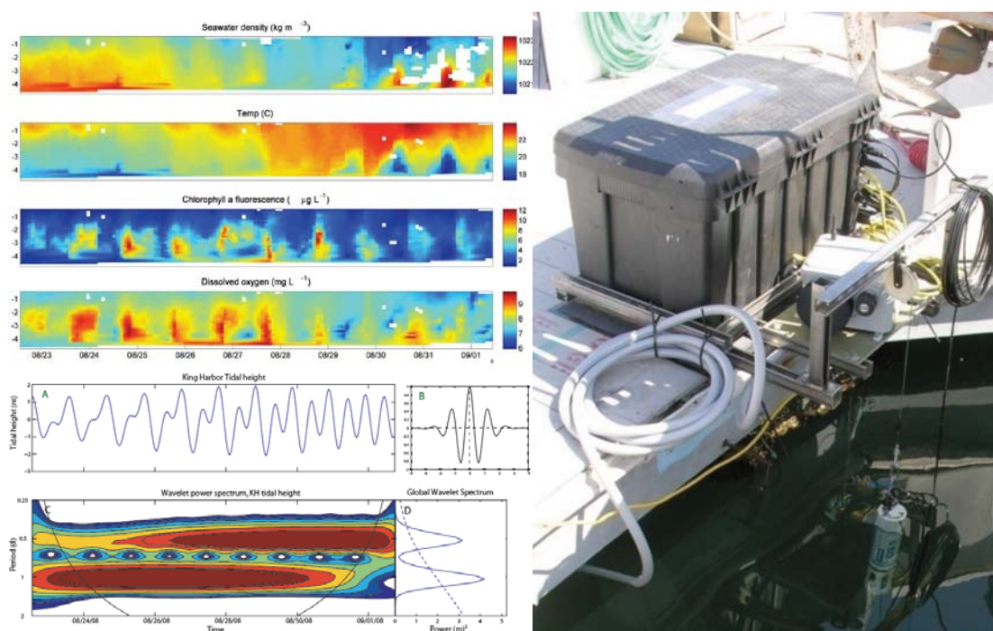
Figure 3. A pier-mounted winch system for characterizing the vertical distribution of chemical, physical, and biological parameters in King Harbor (right panel). Embedded networks yield high-resolution spatiotemporal measurements in aquatic ecosystems. Color contours (4 upper left panels) display a time series of depth-resolved chemical and biological parameters in King Harbor. Wavelet power spectrum analysis of a tidal record (left, middle panel) reveals a strong daily and semi-daily periodicity (dark red bands; left, bottom panel). Strong physical forcing affects the biology of the ecosystem directly by transporting cells, and also by changing light and nutrient availability.
